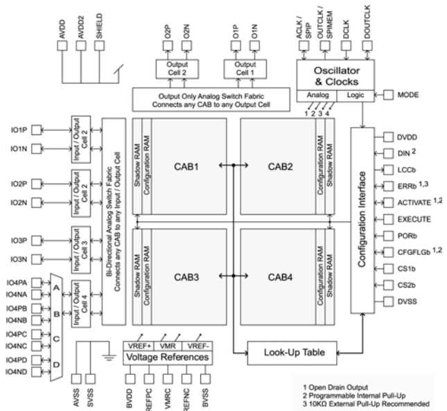
Figure 1: Architectural overview of the AN121E04 device
